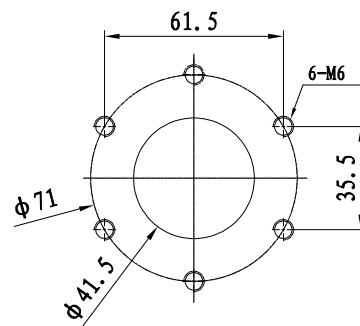
面板安装尺寸 Panel Cut-out
