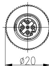
针位排布图 Contact arrangement
