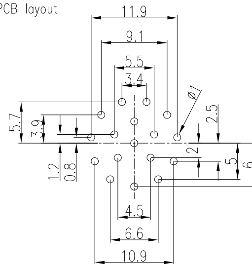
PCB孔细节 PCB layout
