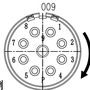
针位排布图 Contact arrangement
