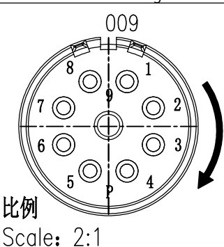
针位排布图 Contact arrangement
