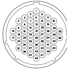
针位排布图 Contact arrangement
