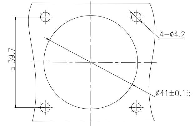
面板安装尺寸 Panel Cut-out
