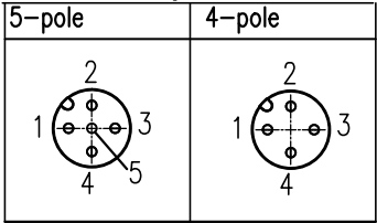
Contact arrangement
