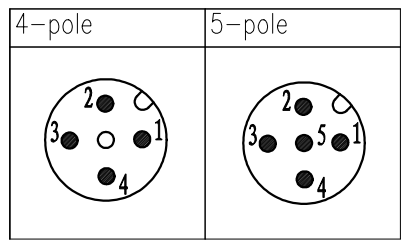
针位排布图 Contact arrangement
