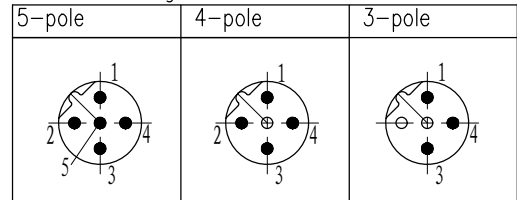
Contact arrangement
