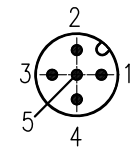
针位排布图 Contact arrangement
