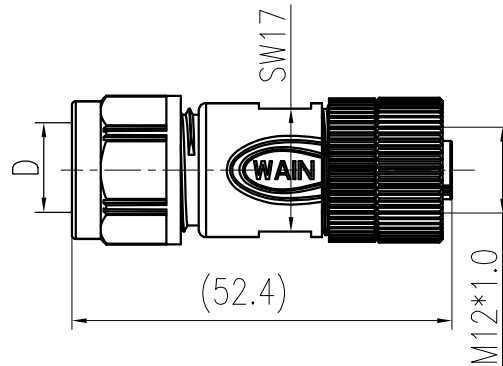
针位排布图 Contact arrangement
