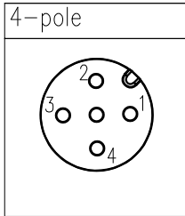
针位排布图 Contact arrangement
