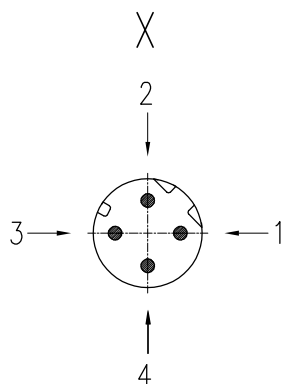
针位图 Contact arrangements
