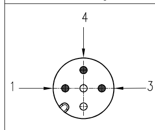
针位图 Contact arrangements
