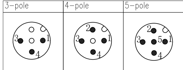
针位排布图 Contact arrangement
