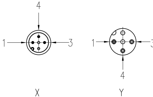
针位图 Contact arrangement
