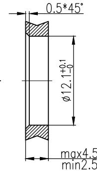
通孔安装 With bore hole
