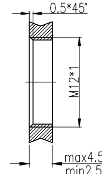
螺纹安装 With thread to screw in
