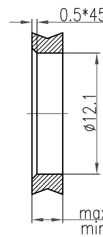
通孔安装 With bore hole
