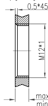
螺纹安装 With thread to screw in
