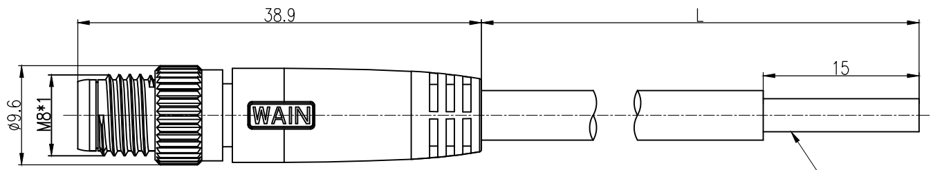
剥线长度 Stripping length of the sheath
