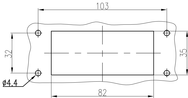
面板开孔图 Panel cut out
