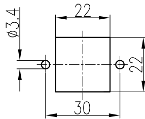
面板开孔图 Panel cut out
