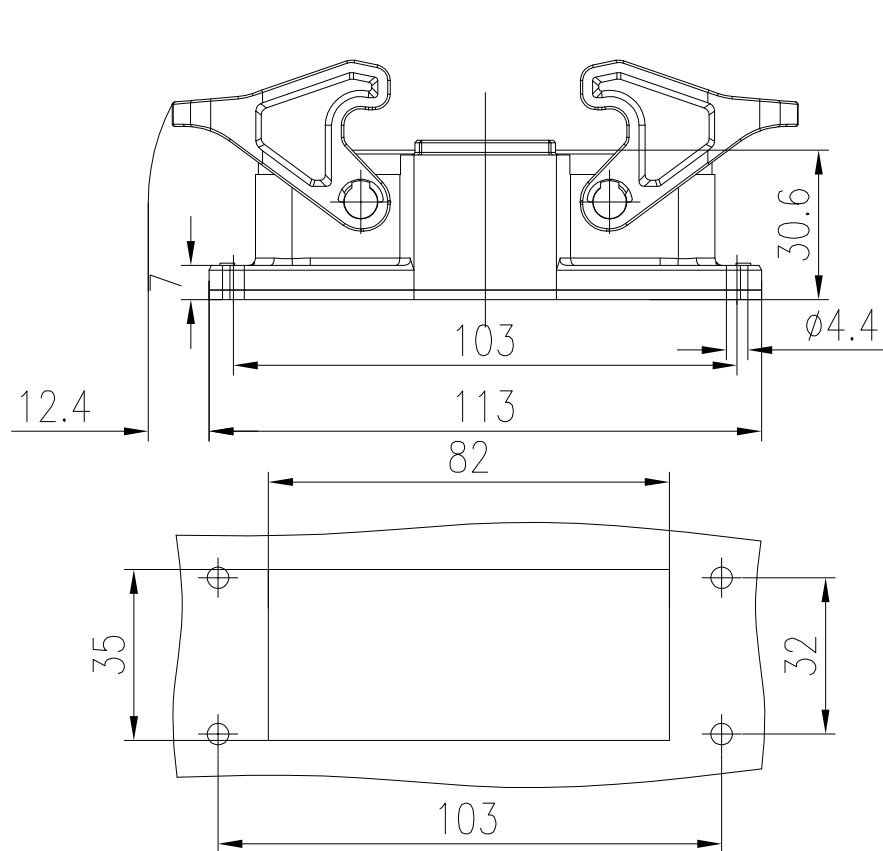
面板开孔图 Panel cut out
