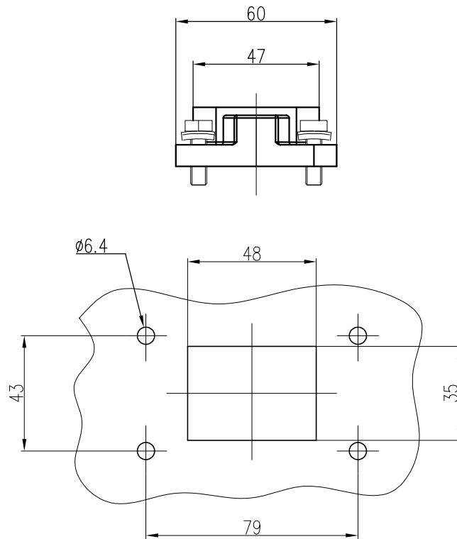
面板开孔图 Panel cut out
