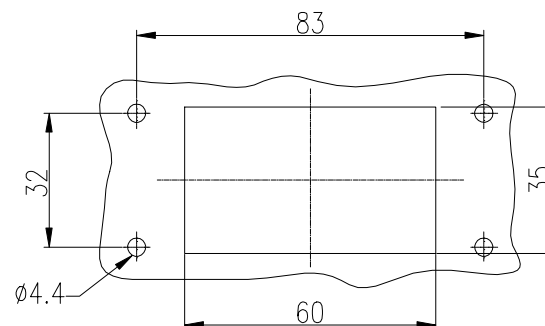
面板开孔图 Panel cut out
