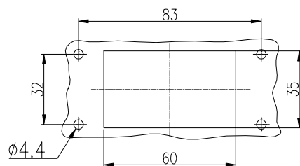
面板开孔图 Panel cut out
