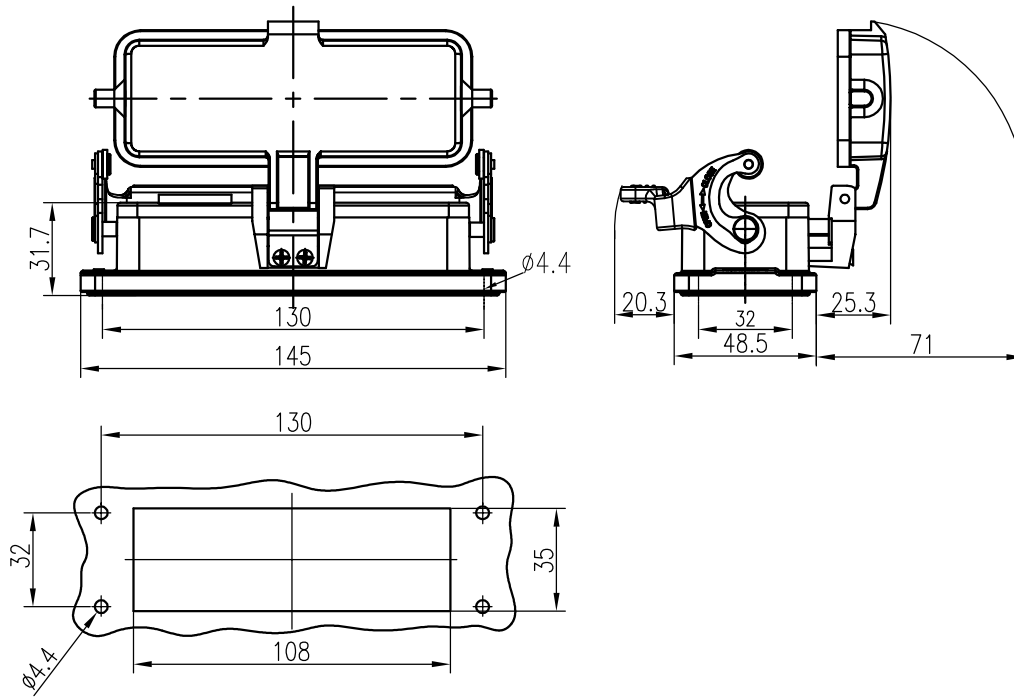
面板开孔图 Panel cut out
