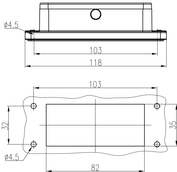
面板开孔图 Panel cut out
