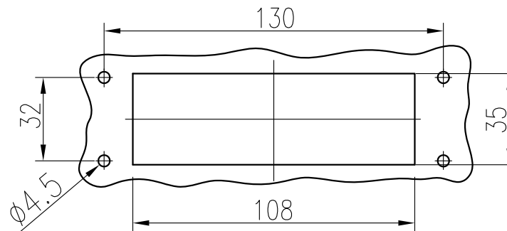
面板开孔图 Panel cut out
