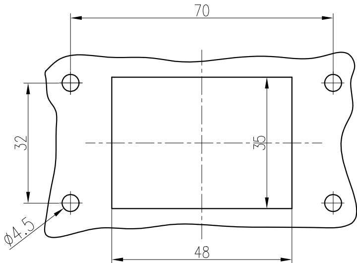
适用的面板开孔图 Applicable Panel cut out
