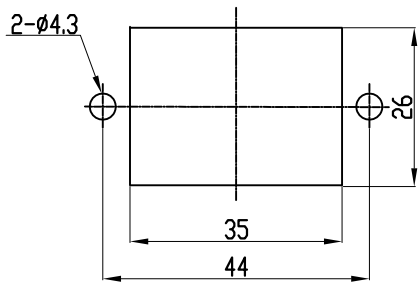
面板安装开孔及两处锁紧尺寸 Panel installation opening and two locking dimensions
